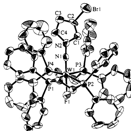
Figure 4. ORTEP drawing for [WF(NNCH=CBrCH=CH)(dppe) 2 ] + ( 7b + ). Hydrogen atoms are omitted for clarity.
