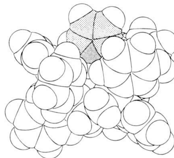
Figure 3. Van der Waals sphere of complex 3b + .
