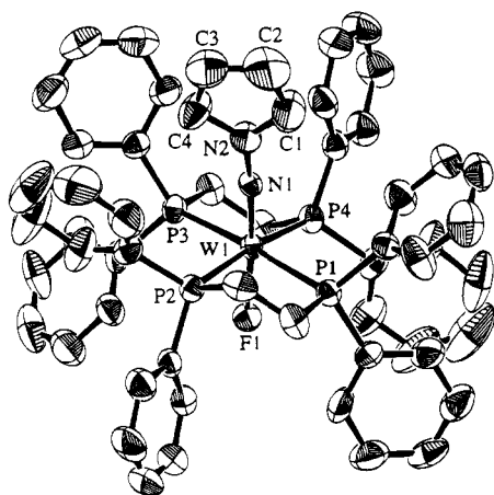
Figure 1. ORTEP drawing for [\text{WF}(\text{NNCH}=\text{CHCH}=\text{CH})(\text{dppe})_2]^+ ( 3b^+ ). Hydrogen atoms are omitted for clarity.
