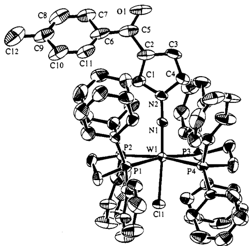
Figure 6. ORTEP drawing for [\text{WCl}\{\text{NNCH}=\text{C}(\text{COC}_6\text{H}_4\text{CH}_3\text{-p})\text{-CH}=\text{CH}\}(\text{dppe})_2]^+ ( 19c + ). Hydrogen atoms are omitted for clarity.
