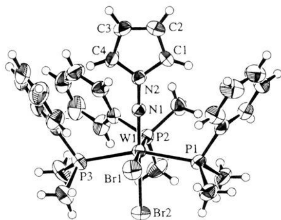
Figure 2. ORTEP drawing for [\text{WBr}_2(\text{NNCH}=\text{CHCH}=\text{CH})(\text{PMe}_2\text{-Ph})_3] ( 6b ).
