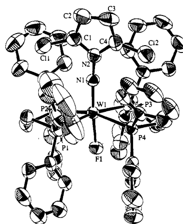
Figure 5. ORTEP drawing for [WF(NNCCI=CHCH=CCI)(dppe) 2 ] + ( 13b + ). Hydrogen atoms are omitted for clarity.
